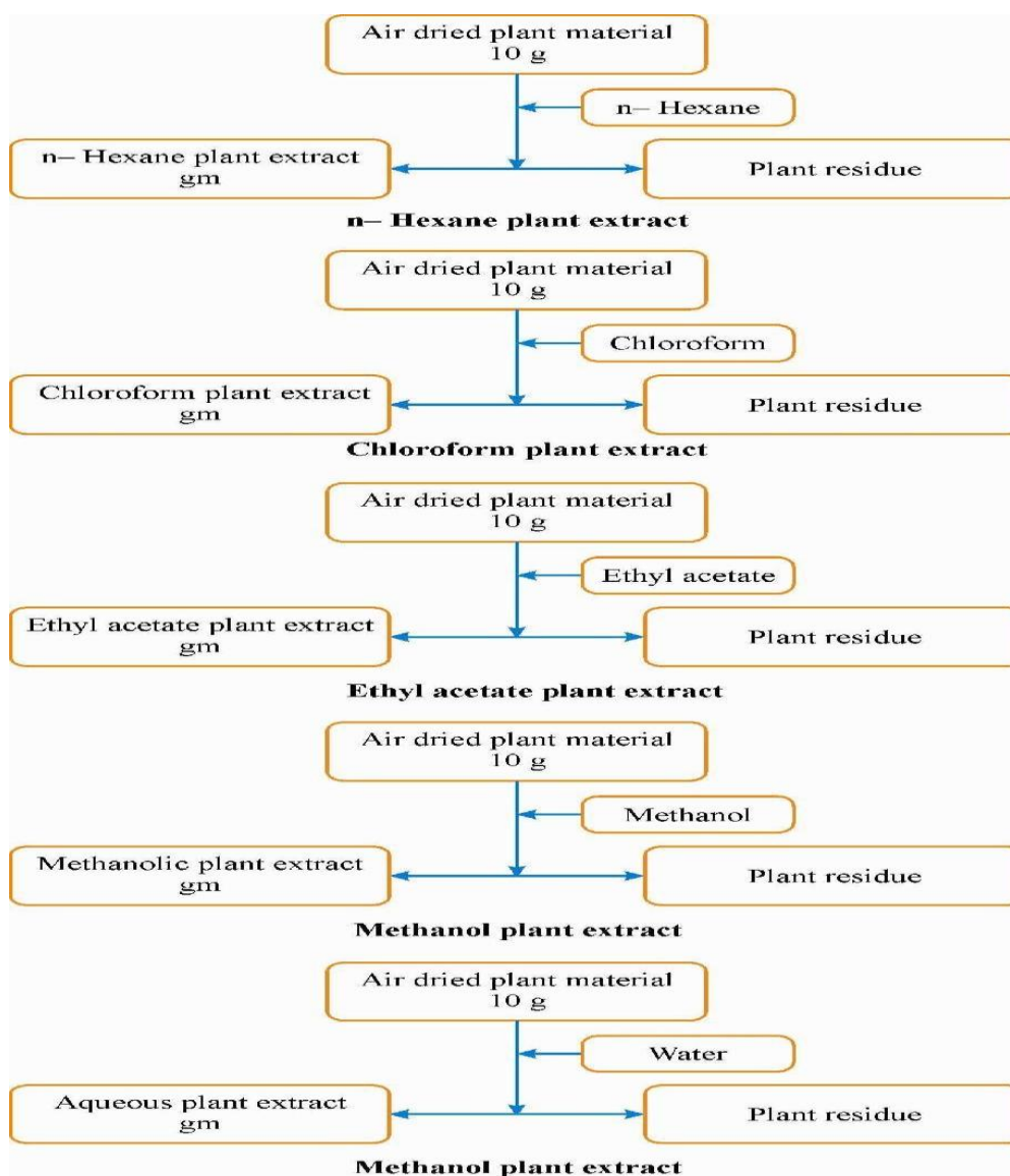
FIG. 1: Flow chart for preparation of plant extracts by Soxhlet extraction method
