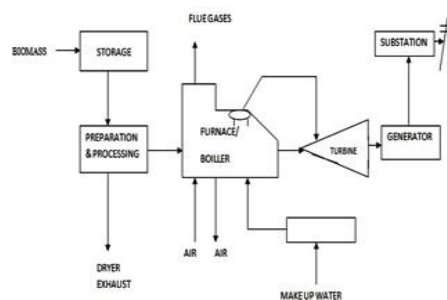
Figure 4.1 block diagram of direct firing
