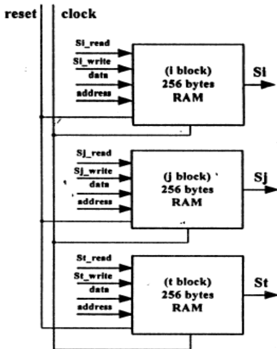
FIGURE 4 THE S-BOX RAM
