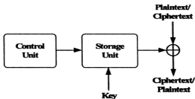
FIGURE 2 BLOCK DIAGRAM OF RC4 STREAM CIPHER.
