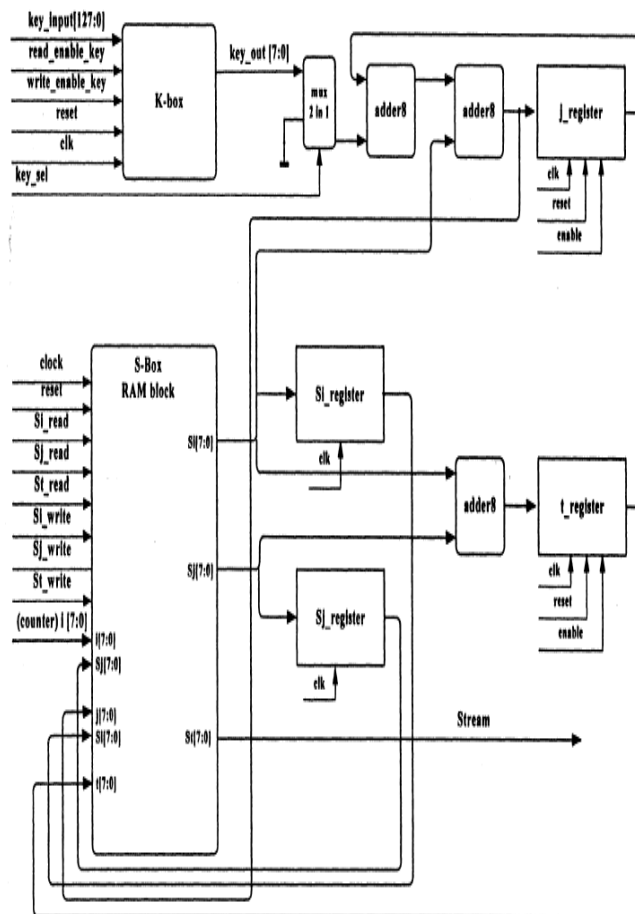
FIGURE 3 STORAGE UNIT IMPLEMENTATION
