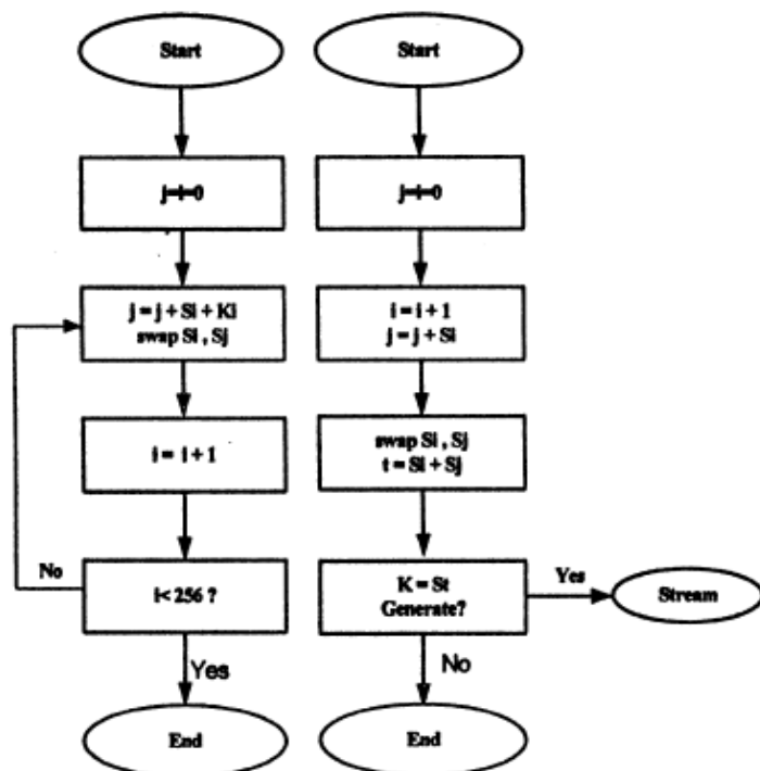
FIGURE 1 BLOCK DIAGRAM OF RC4 PHASES.
