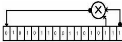
Figure 2.4: Linear Feedback Shift Register (LFSR)
