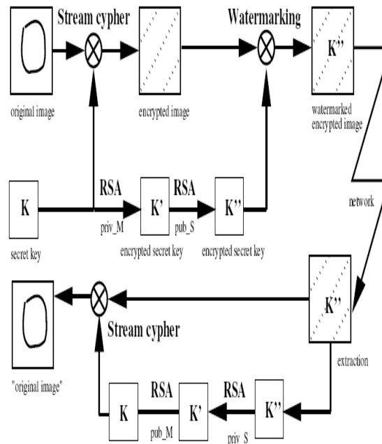
Figure 3: Combination of public key encryption, secret key encryption, and watermarking
