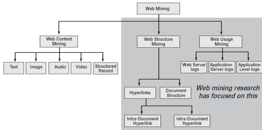
Taxonomy of web mining
