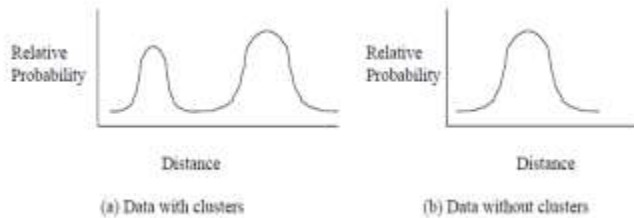
Figure 2: Plot of distances between points for grouped and ungrouped data
