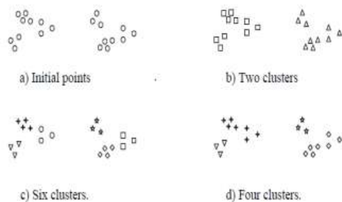
Figure 1: Various classifications for the same collection of points
