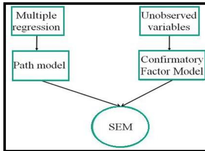
Fig 1 Pre-requisites of Structural Equation Modeling
