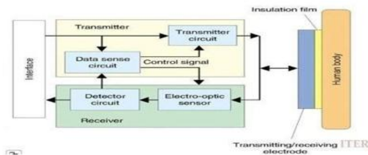
Fig 1: Block diagram of RedTacton Transceiver (Source: Modak et al. 2020)
